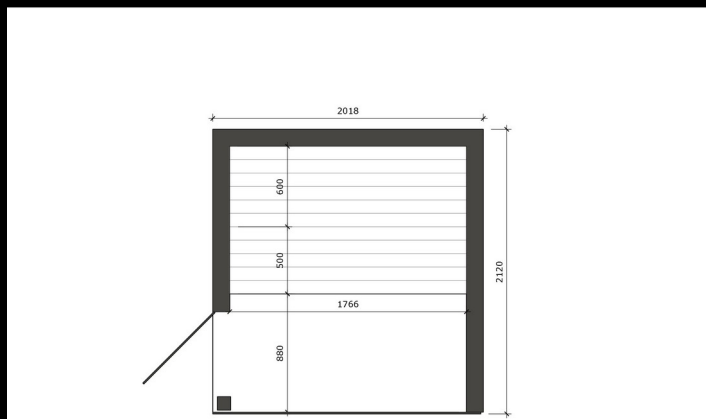
Floor plan — dimensions in mm. Door available left or right hinged.
